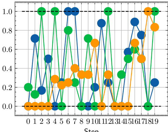
MulticlassRecallAtFixedPrecision
