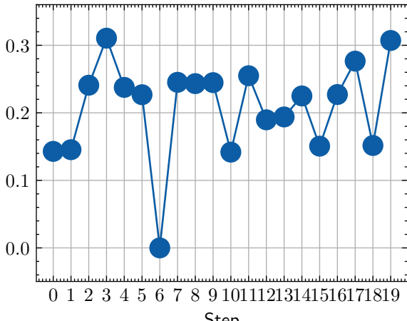
IntersectionOverUnion
