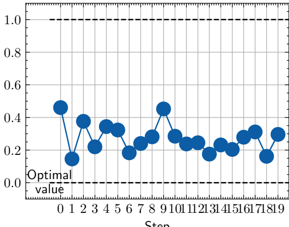
MulticlassCalibrationError
