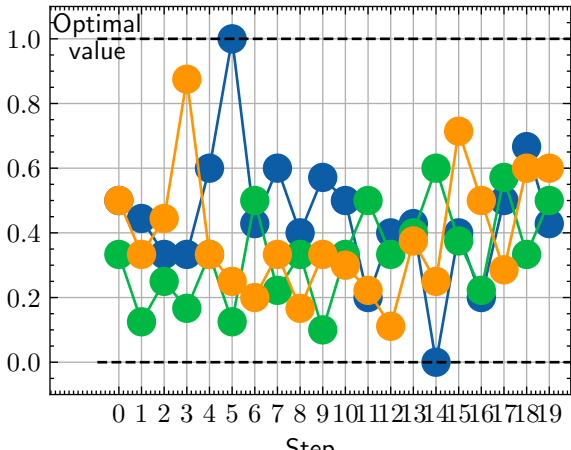
MulticlassAccuracy
