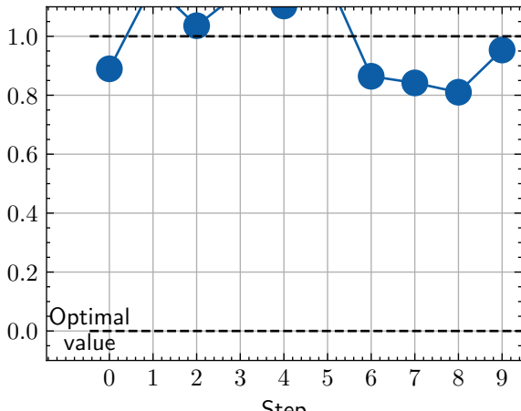
BinaryHingeLoss
