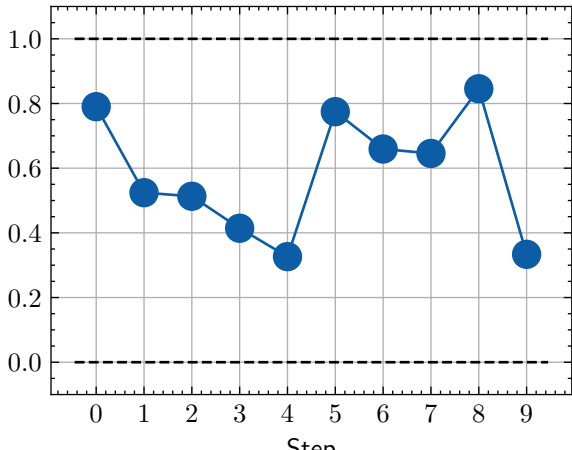
BinaryAveragePrecision
