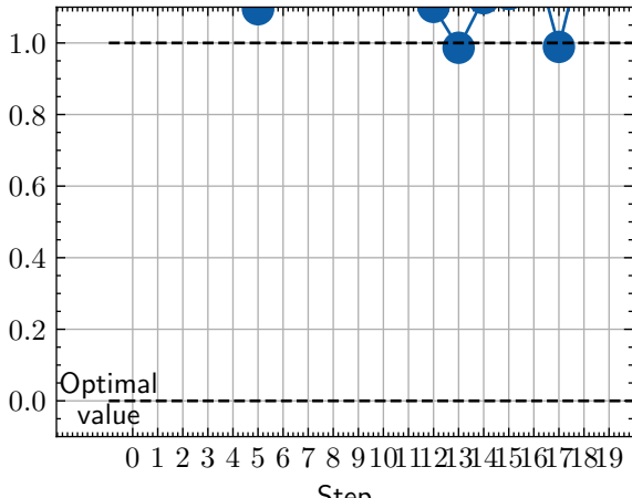
MulticlassHingeLoss
