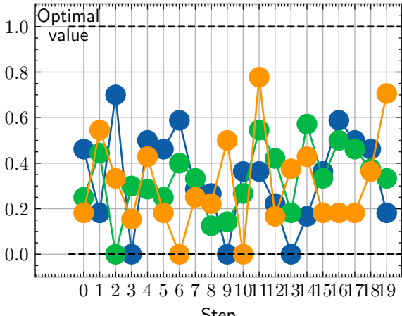
MulticlassF1Score
