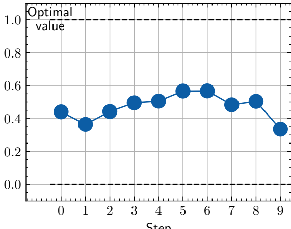
MultilabelFBetaScore
