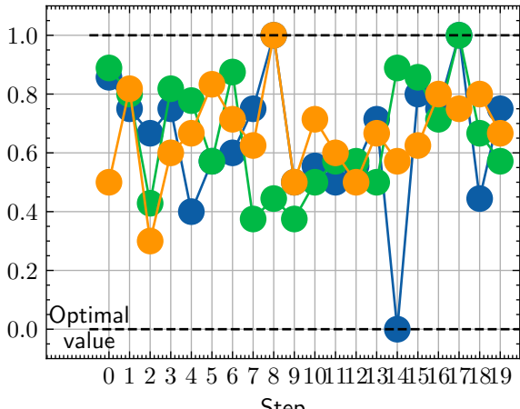
MulticlassHammingDistance
