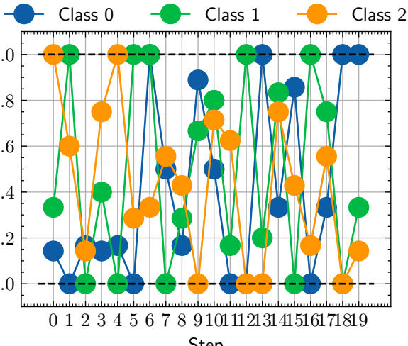
MulticlassRecallAtFixedPrecision
